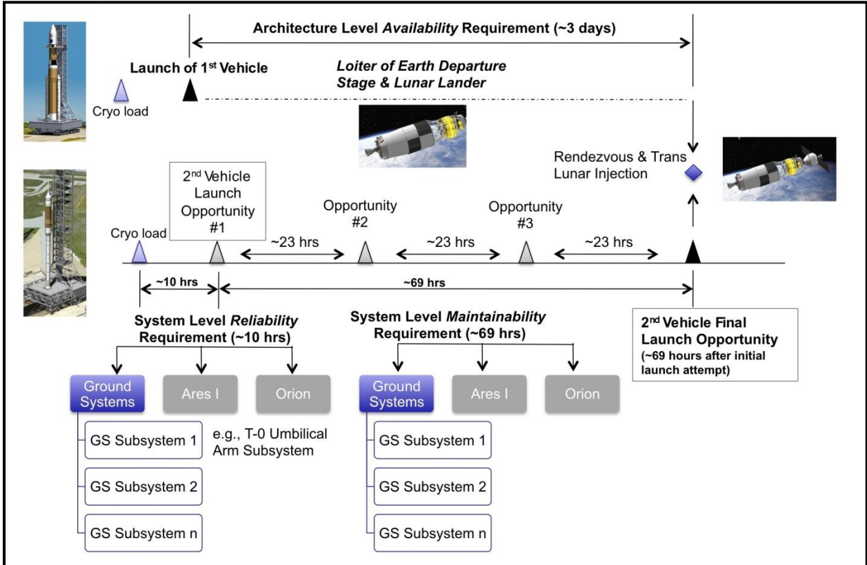
Figure 1. Constellation 2-Launch Lunar Architecture and the Associated Launch Probability Requirements Flow to Ground Subsystems
